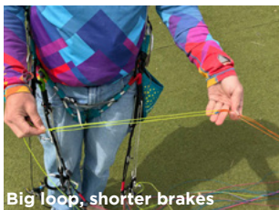
Big loop, shorter brakes
