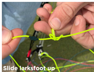
Slide larksfoot up
